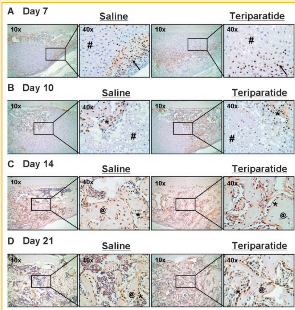
Fig. 3. The effects of teriparatide on Osx protein expression during fracture repair. Seven- to nine-week-old C57BL/6 mice underwent unilateral femur fractures and were subsequently injected daily with teriparatide (right panels; 10× and 40×) or saline solution (left panels; 10× and 40×) as described in Materials and Methods Section. Osx proteins were detected in the fracture callus at days 7(A), 10(B), 14(C), and 21(D) post-fracture using immunohistochemical analysis. Of note is the strong immunostaining in the progenitor cells (arrows) as well as osteoblasts (*) and osteocytes (@) seen in newly formed bone. In addition, there is a lack of staining in the hypertrophic chondrocytes (#).
