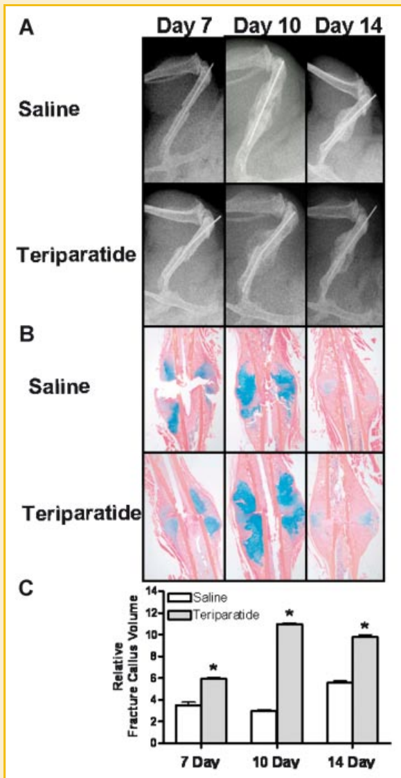
Fig. 2. Teriparatide accelerates femur fracture repair. Seven- to nine-week-old C57BL/6 mice underwent unilateral femur fractures and were subsequently injected with daily teriparatide (lower panels) or saline solution (upper panels) as described in Materials and Methods Section. X-rays (A), histology (B), and histomorphometric analysis (C) were performed 7, 10, and 14 days post-fracture. Values are expressed as means \pm SE ( n = 3 ). * denotes statistical significance from controls at each time point ( P < 0.05 ). [Color figure can be viewed in the online issue, which is available at www.interscience.wiley.com .]
